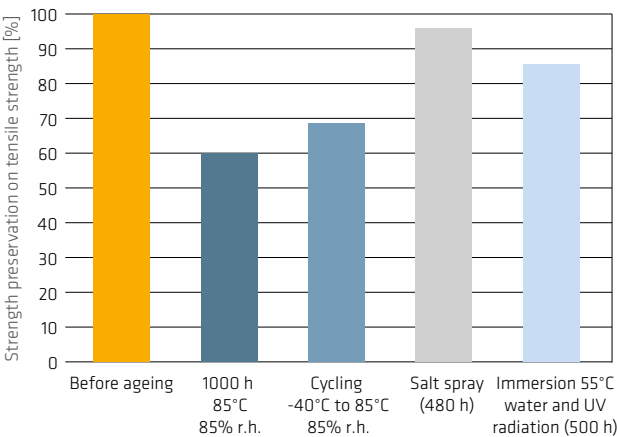
Strength preservation after exposure
